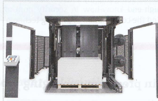
The BSW_AUM pile turner, specifically designed for non-stop automatic sheetfed printing and stamping machines
